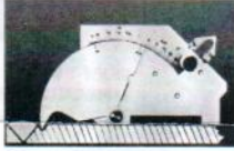
Fillet Weld Throat
